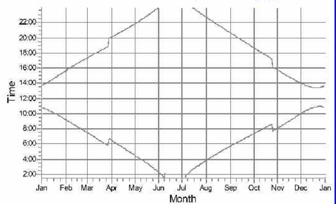
8: NORDEX N117 hub: 120.0 m (TOT: 178.5 m) (8)
