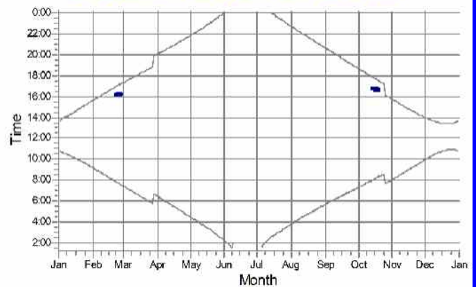
24: NORDEX N117 hub: 120.0 m (TOT: 178.5 m) (24)
