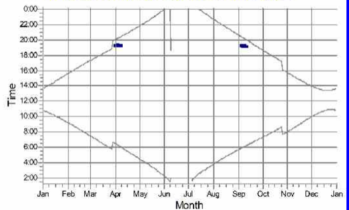
22: NORDEX N117 hub: 120.0 m (TOT: 178.5 m) (22)
