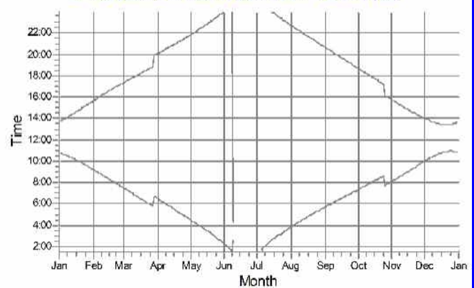
18: NORDEX N117 hub: 120.0 m (TOT: 178.5 m) (18)
