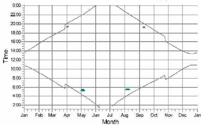
7: NORDEX N117 hub: 120.0 m (TOT: 178.5 m) (7)
