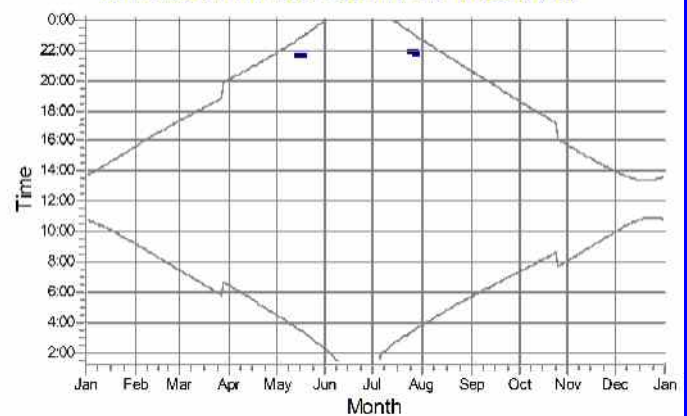
16: NORDEX N117 hub: 120.0 m (TOT: 178.5 m) (16)
