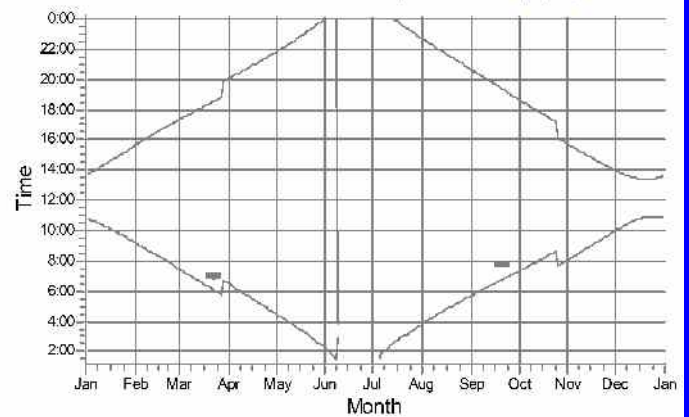
26: NORDEX N117 hub: 120.0 m (TOT: 178.5 m) (26)
