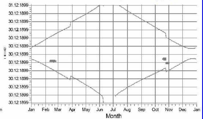
14: NORDEX N117 hub: 120.0 m (TOT: 178.5 m) (14)
