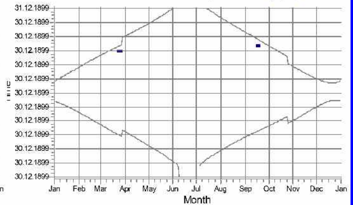
50: NORDEX N117 hub: 120.0 m (TOT: 178.5 m) (50)
