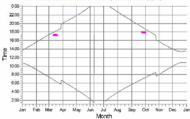
41: NORDEX N117 hub: 120.0 m (TOT: 178.5 m) (41)
