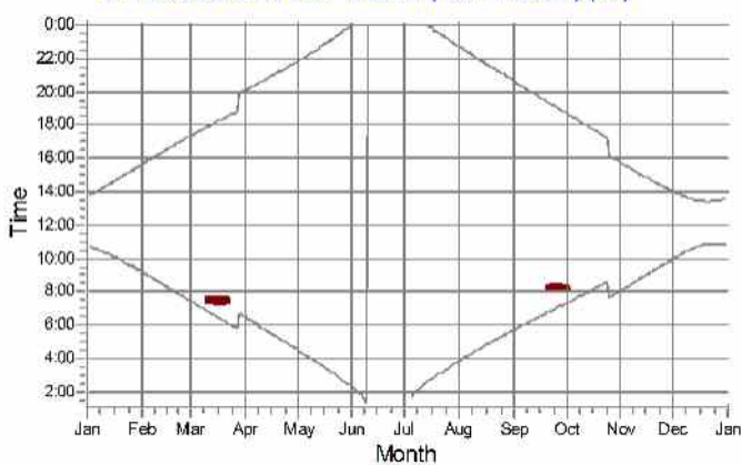
47: NORDEX N117 hub: 120.0 m (TOT: 178.5 m) (47)
