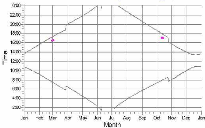
43: NORDEX N117 hub: 120.0 m (TOT: 178.5 m) (43)
