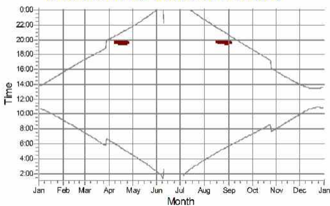
45: NORDEX N117 hub: 120.0 m (TOT: 178.5 m) (45)
