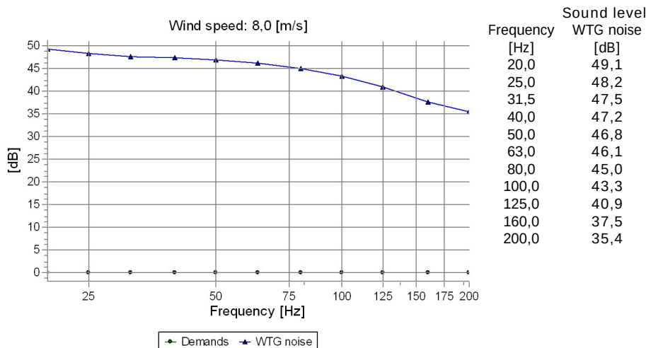
F Noise sensitive point: Finnish low frequency - User defined (4)
