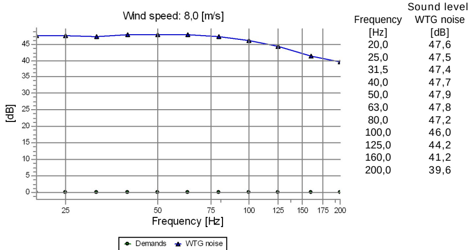
E Noise sensitive point: Finnish low frequency - User defined (7)
