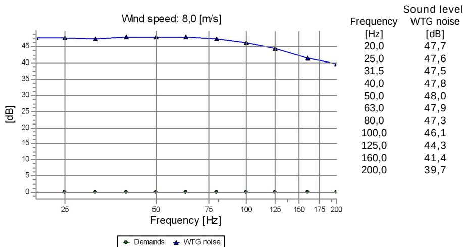
F Noise sensitive point: Finnish low frequency - User defined (4)
