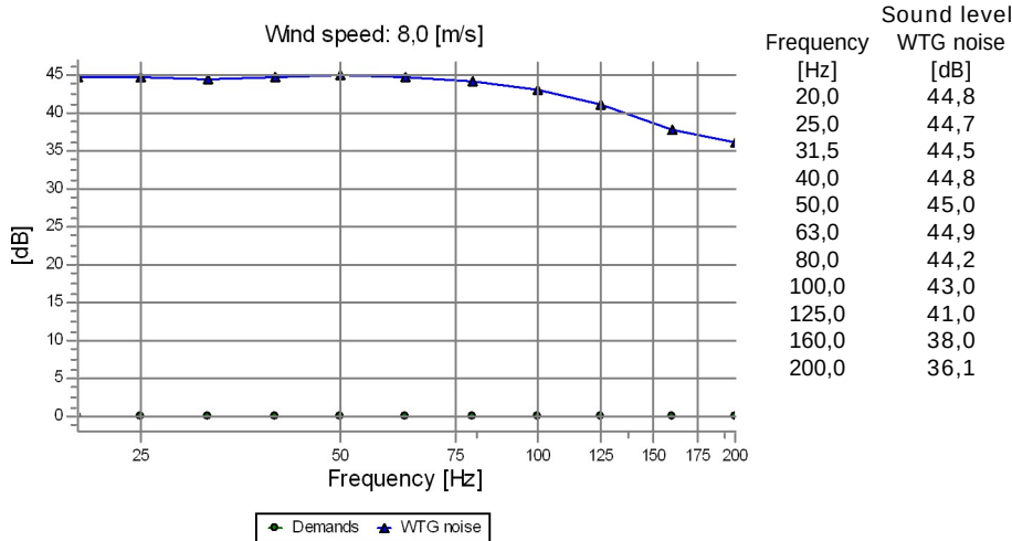
B Noise sensitive point: Finnish low frequency - User defined (1)
