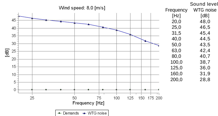
H Noise sensitive point: Finnish low frequency - User defined (5)
