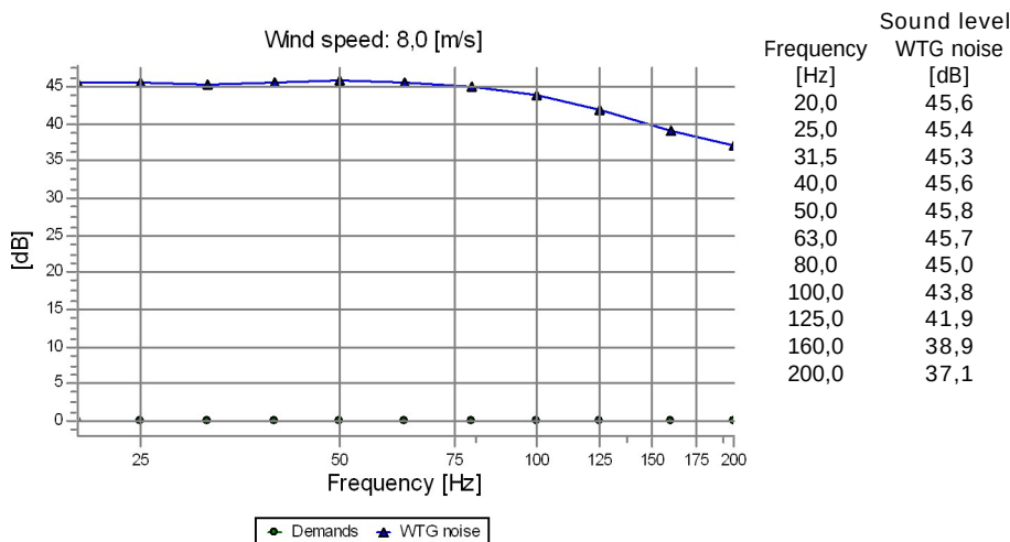
B Noise sensitive point: Finnish low frequency - User defined (1)
