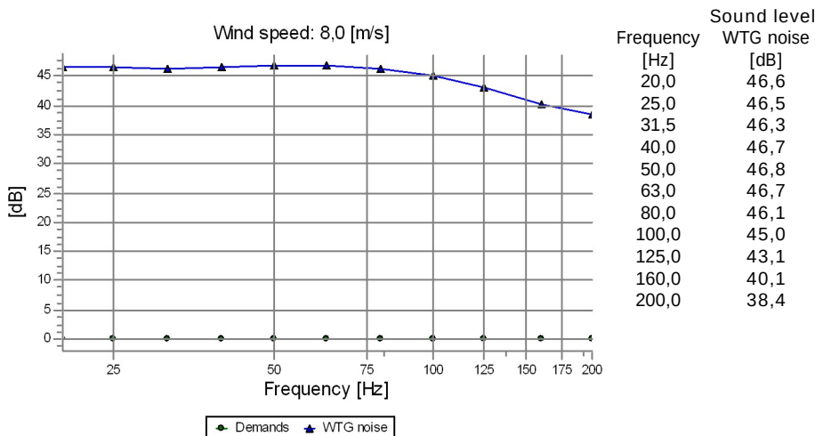
C Noise sensitive point: Finnish low frequency - User defined (8)
