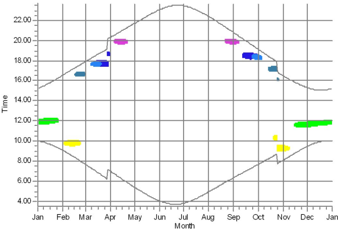
7: Shadow Receptor: 1,0 × 1,0 Azimuth: 0,0° Slope: 90,0° (7)
