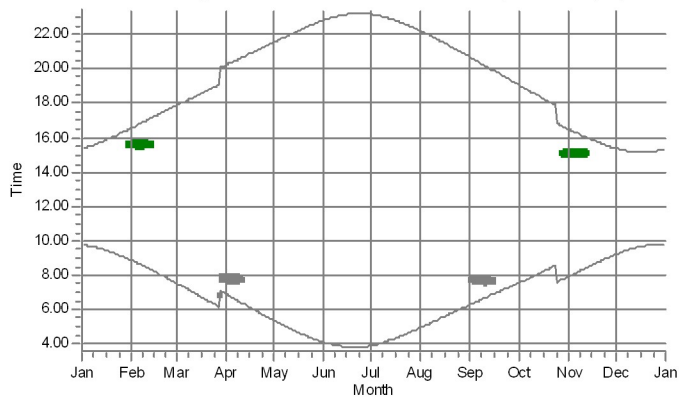
7: Shadow Receptor: 1.0 × 1.0 Azimuth: 0.0° Slope: 90.0° (93)
