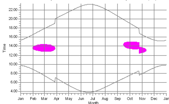
4: Shadow Receptor: 1.0 × 1.0 Azimuth: 0.0° Slope: 90.0° (90)
