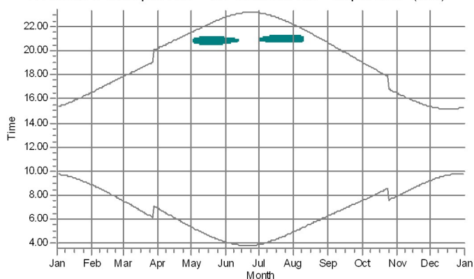
17: Shadow Receptor: 1.0 × 1.0 Azimuth: 0.0° Slope: 90.0° (103)
