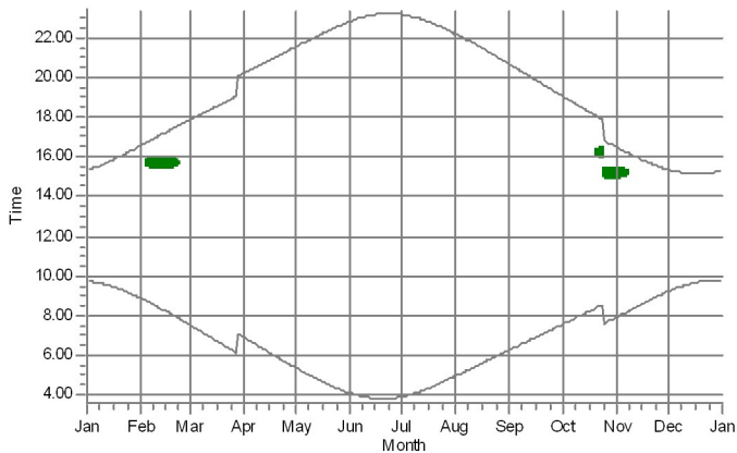
7: Shadow Receptor: 1.0 x 1.0 Azimuth: 0.0  Slope: 90.0  (93)
