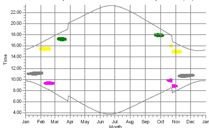
6: Shadow Receptor: 1.0 × 1.0 Azimuth: 0.0° Slope: 90.0° (92)
