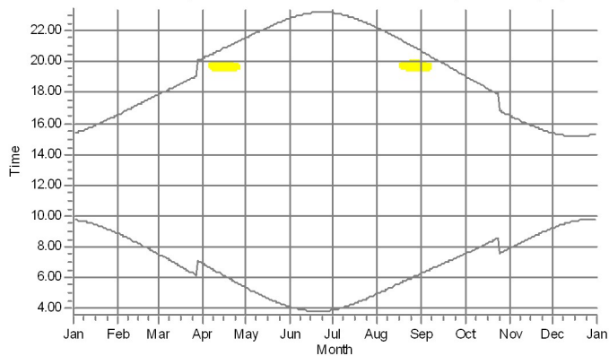
13: Shadow Receptor: 1.0 × 1.0 Azimuth: 0.0° Slope: 90.0° (99)
