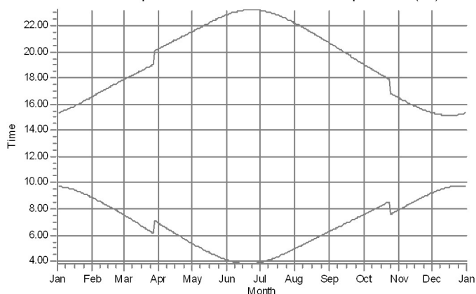
3: Shadow Receptor: 1.0 × 1.0 Azimuth: 0.0° Slope: 90.0° (89)
