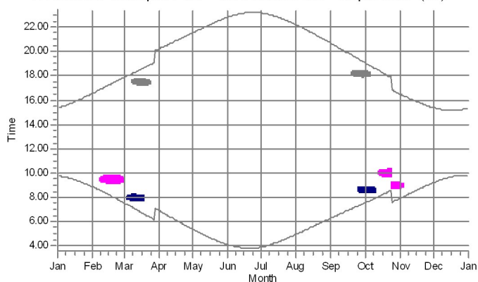
11: Shadow Receptor: 1.0 × 1.0 Azimuth: 0.0° Slope: 90.0° (97)
