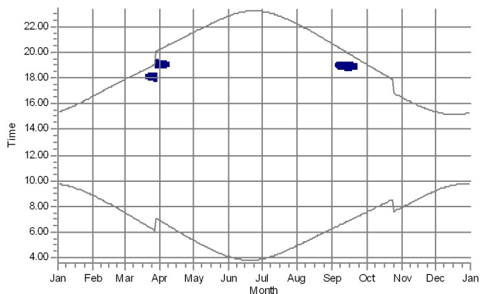
1: Shadow Receptor: 1.0 × 1.0 Azimuth: 0.0° Slope: 90.0° (87)
